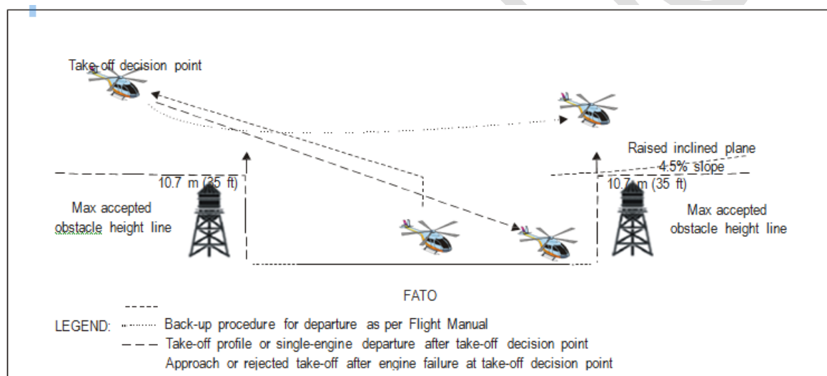
Figure 14 - Example of raised inclined plane during operations in Performance Class 1 (ICAO Annex 14, Vol II Figure 4.4)
