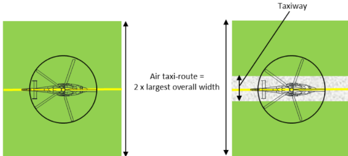
Figure 4 - Helicopter air taxi-route and combined air taxi-route/taxiway (ICAO Annex 14, Vol II Figure 3.4)
