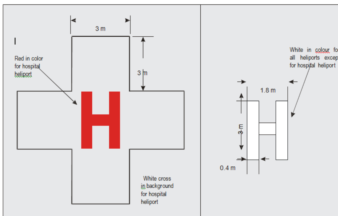
Figure 26 - Hospital heliport identification and heliport identification marking (ICAO Annex 14, Vol II Figure 5.4)
