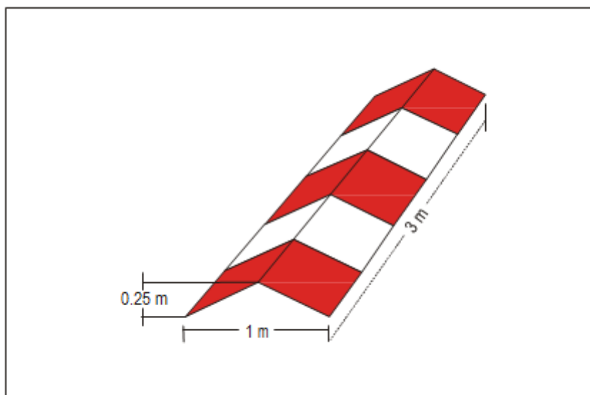
Figure 28 - Runaway type FATO edge marker ( ICAO Annex 14, Vol II Figure 5.6)
