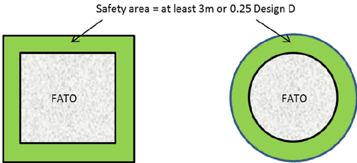
Figure 1 - FATO and associate safety area (ICAO Annex 14 Vol II Fig 3-1)
