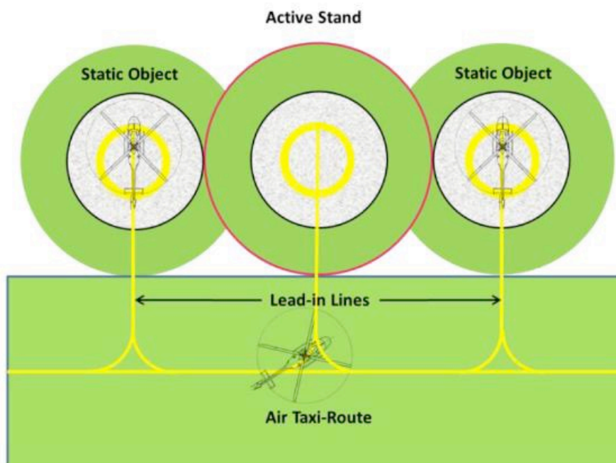
Figure 9 – Turning stands (with air taxi-routes) non-simultaneous use – inner stands active (ICAO Annex14, Vol II Fig 3.9)
