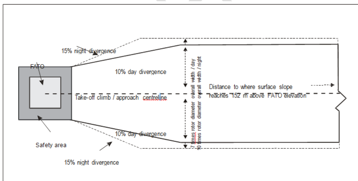
Figure 11 - Obstacle limitation surfaces -- Take-off climb and approach surface (ICAO Annex 14, Vol II Figure 4.1)
