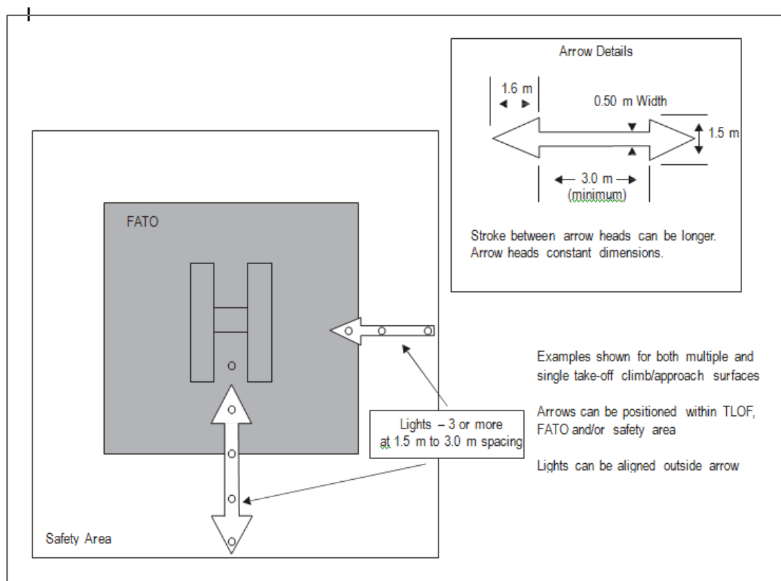
Figure 32 - Flight path alignment guidance markings and lights (ICAO Annex 14, Vol II Figure 5.10)
