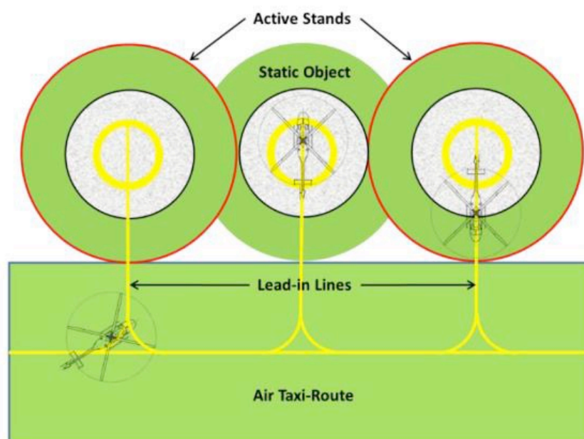
Figure 8 – Turning stands (with air taxi-routes) non-simultaneous use – outer stands active (ICAO Annex14, Vol II Fig 3.8)
