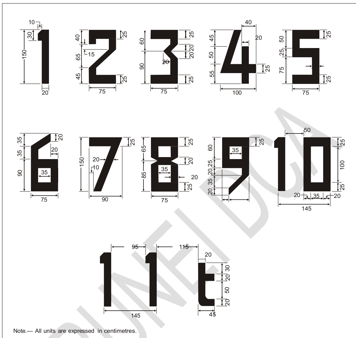
Figure 27 - Form and proportions of numbers and letters ( ICAO Annex 14, Vol II Figure 5.5)
