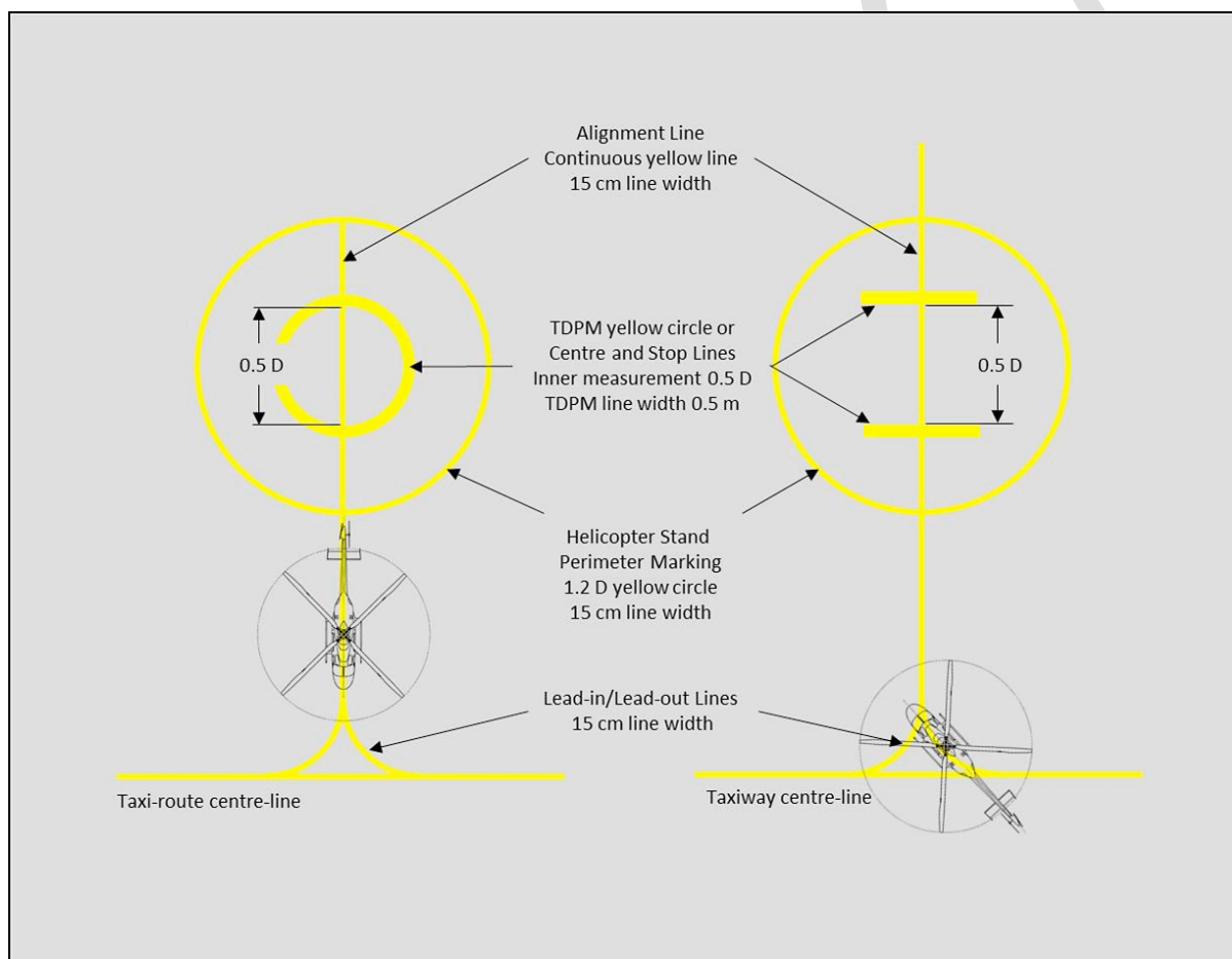
Figure 31 - Helicopter stand markings (ICAO Annex 14, Vol II Figure 5.9)
