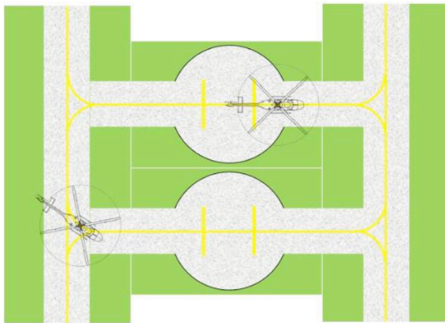
Figure 3 – Ground taxi-through stands (with taxiway/ground taxi-route) simultaneous use (ICAO Annex14, Vol II Fig 3.6)
