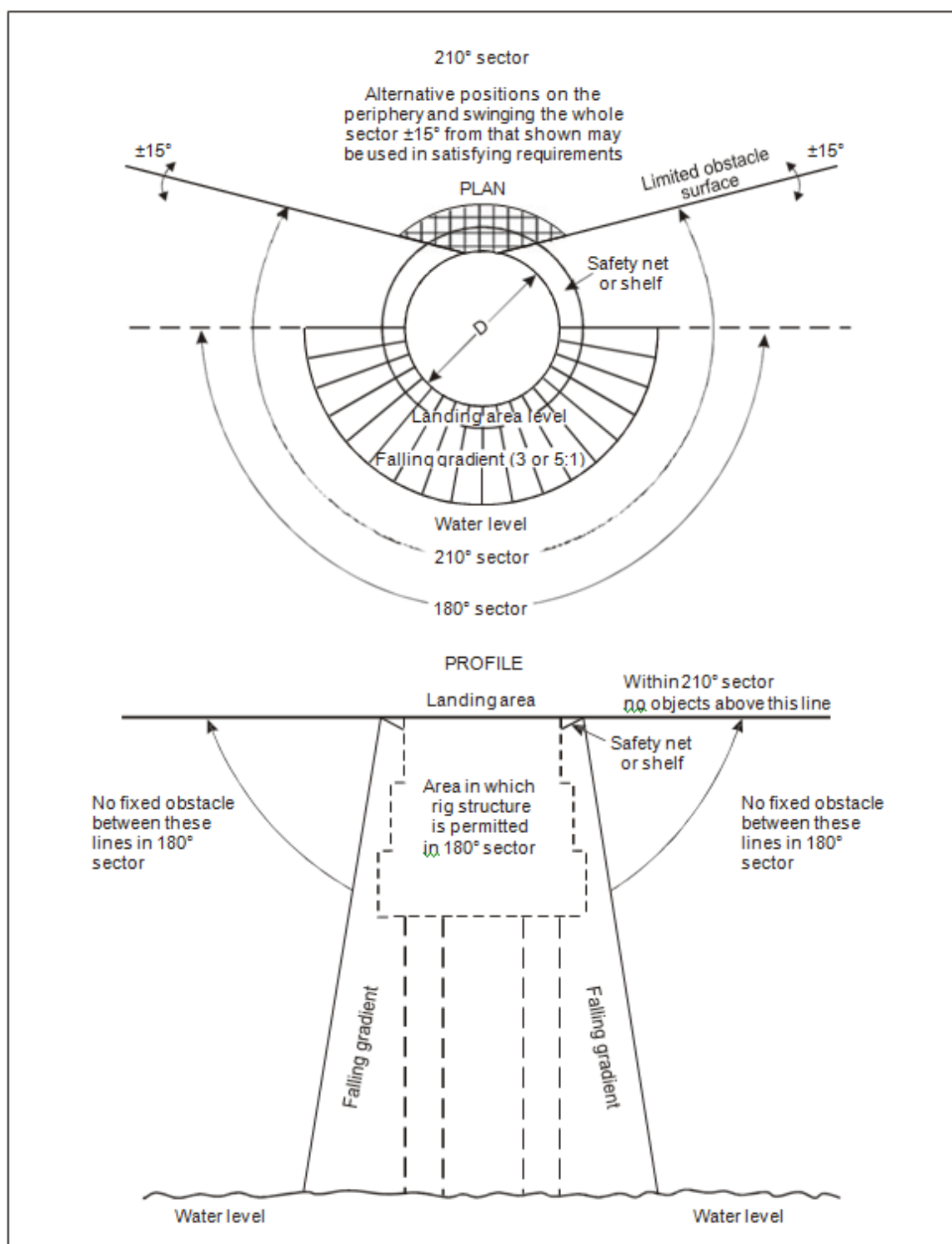
Figure 17 - Helideck obstacle-free sector ( ICAO Annex 14, Vol II Figure 4.7)
