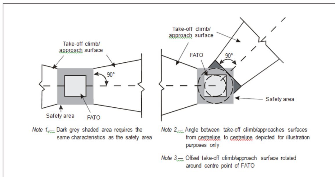
Figure 11 - Obstacle limitation surfaces -- Take-off climb and approach surface (ICAO Annex 14, Vol II Figure 4.1)
