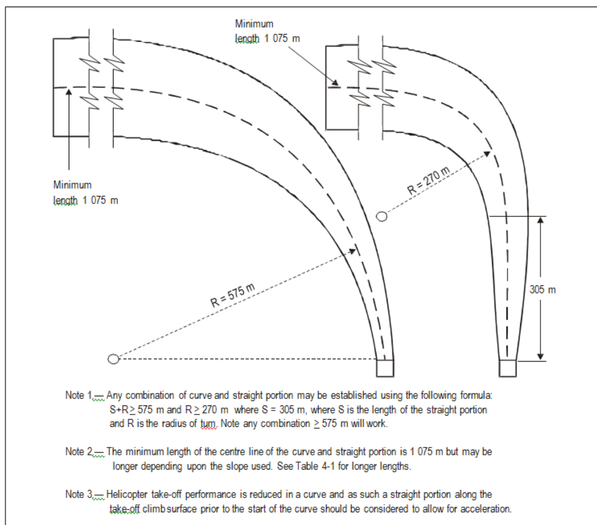
Figure 15 - Curved approach and take-off climb surface for all FATOs (ICAO Annex14, Vol II Figure 4.5)
