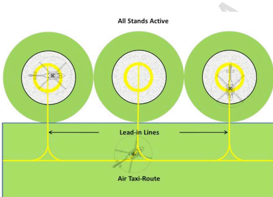
Figure 2 – Turning stands (with air taxi-routes) /simultaneous use (ICAO Annex14, Vol II Fig.3.5)
