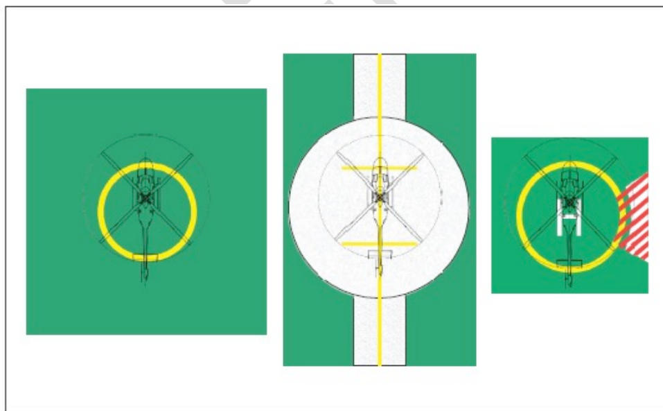
Figure 306 – (Left) multidirectional TDPC with no limitations. (Centre) unidirectional marking shoulder line with associated centreline. (Right) multidirectional TDPC with prohibited landing sector marking (ICAO Annex 14 Vol II Figure 5.8)
