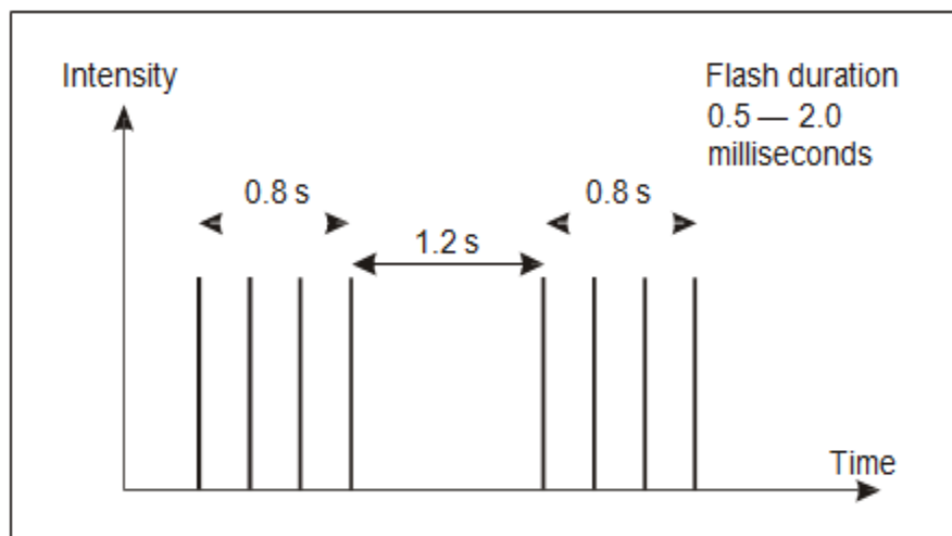
Figure 33 - Heliport beacon flash characteristics ( ICAO Annex Vol II Figure 5.11)
