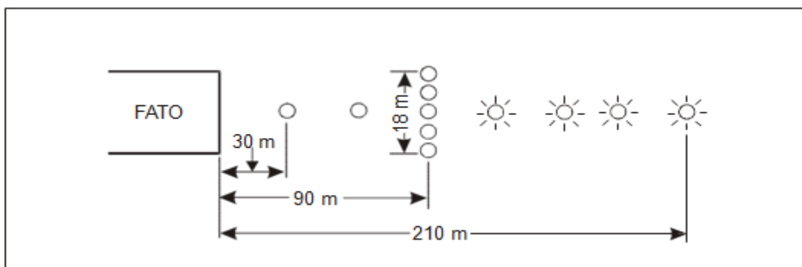
Figure 35 - Approach lighting system (ICAO Annex 14, Vol II Figure 5.13)
