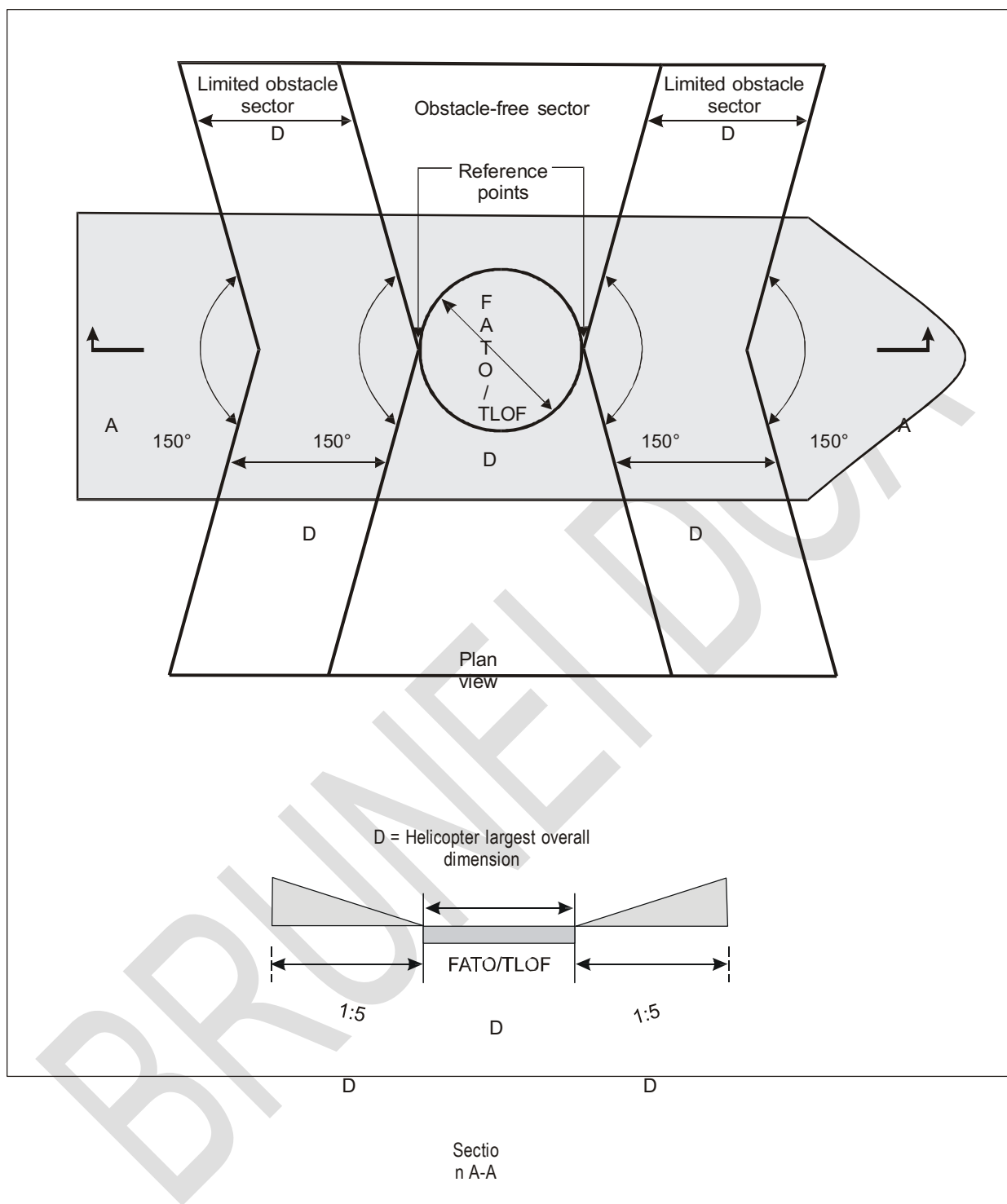
Figure 20 - Amidship's location -- Shipboard heliport obstacle limitation surfaces ( ICAO Annex14, Vol II Figure 4.10)
