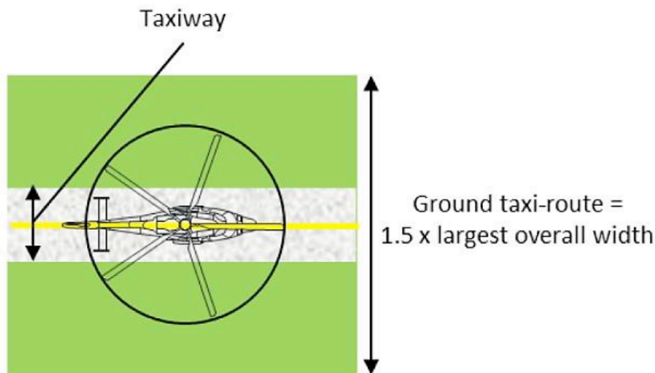
Figure 3 - Helicopter taxiway/ground taxi-routes (ICAO Annex 14, Vol II Fig.3.3)
