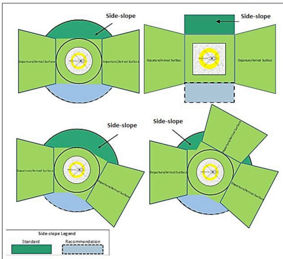
Figure 2 - FATO simple/complex safety area and side slope protection (ICAO Annex 14 Vol II Fig 3-2)
