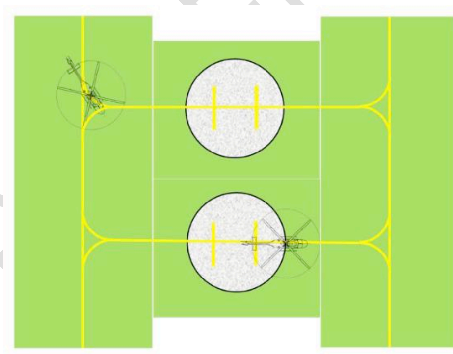
Figure 7 – Air taxi-through stands (with air taxi-route) simultaneous use (ICAO Annex14, Vol II Fig 3.7)
