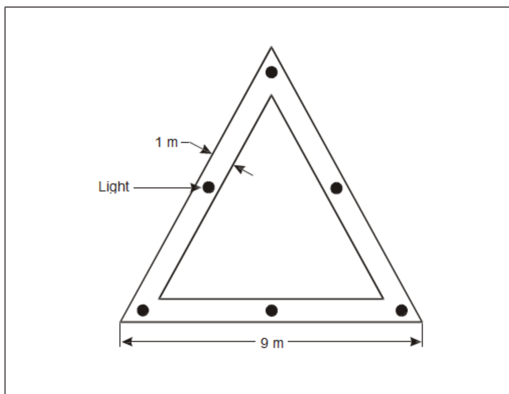
Figure 29 - Aiming point marking (ICAO Annex 14 Vol II Figure 5.7)
