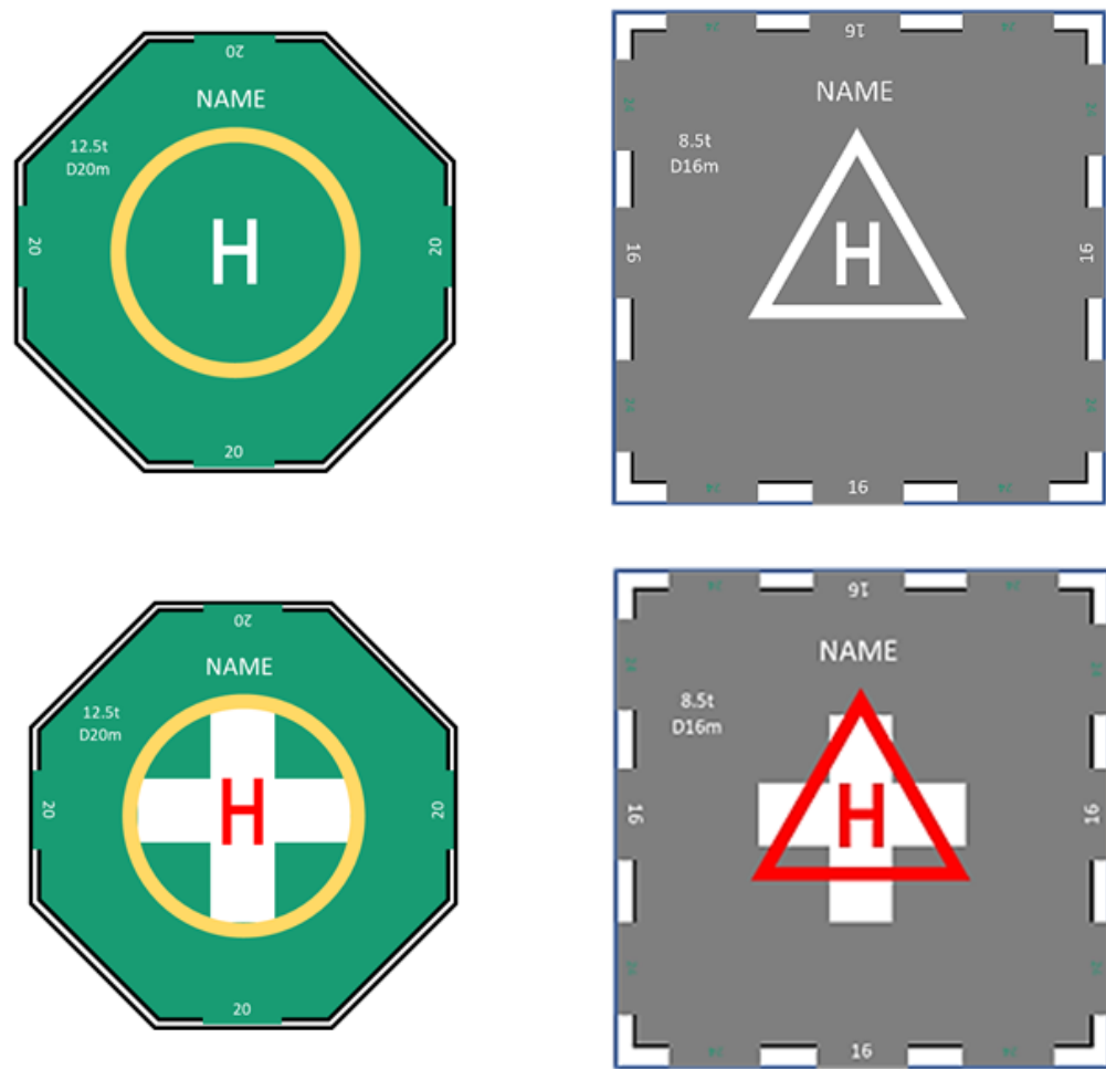
Figure 24 - Heliport identification markings with TLOF and aiming markings for heliport and hospital heliport (ICAO Annex 14, Vol II Figure 5.2)
