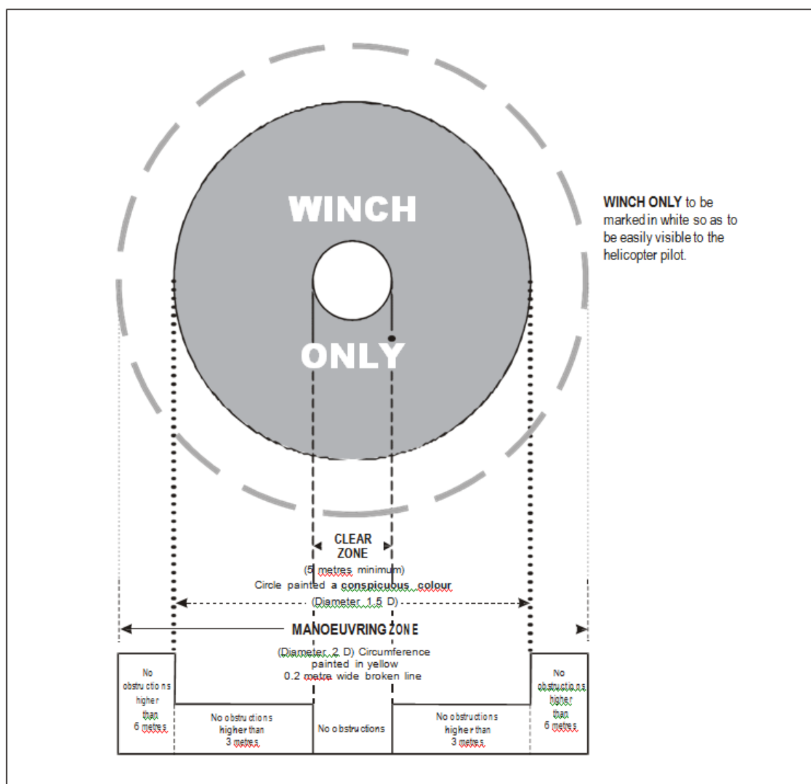
Figure 22 – Winching area of a ship (ICAO Annex 14, Vol II Figure 4.12)
