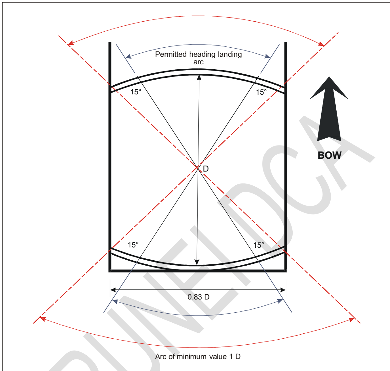
Figure 10 - Shipboard permitted landing headings for limited heading operations (ICAO Annex14, Vol II Fig.3.10)
