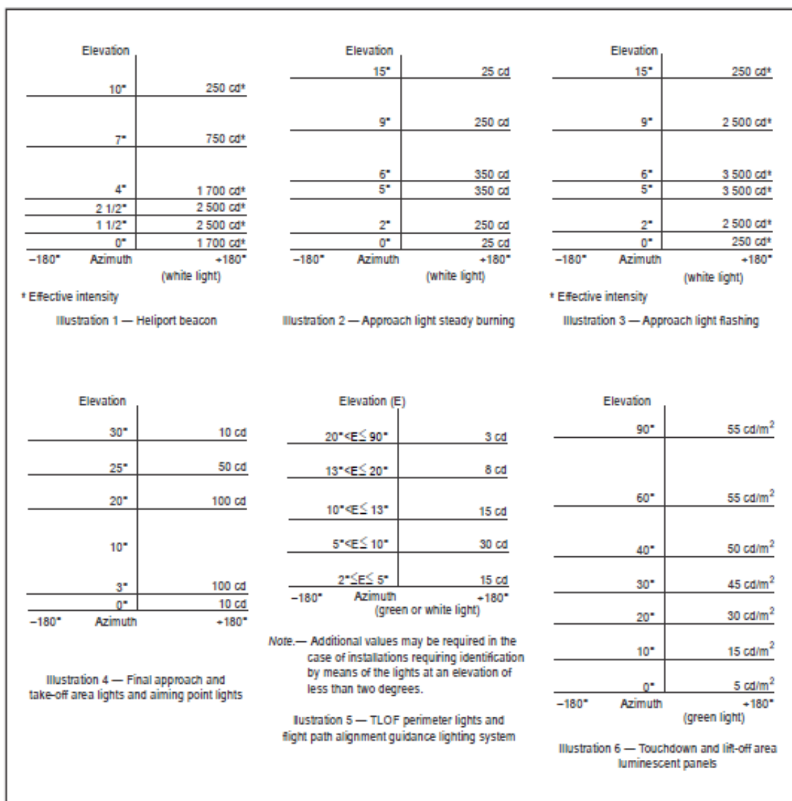
Figure 347 - Isocandela diagrams (ICAO Annex 14, Vol II Figure 5.12)
