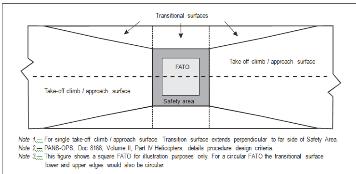
Figure 13 - Transitional surface for a FATO with a PinS approach procedure with a VSS (ICAO Annex 14, Vol II Figure 4.3)
